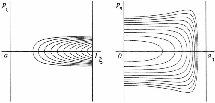
Fig. 7. Phase portrait of billiard motion in a prolate ellipsoid. a = 0.4 , l_\varphi = 0.4 . Equidistant values of \kappa^2 have been chose. Left: intersection of invariant tori with the (\xi, p_\xi) -plane; right: intersection of invariant tori with the (\eta, p_\eta) -plane. There is no separatrix.
