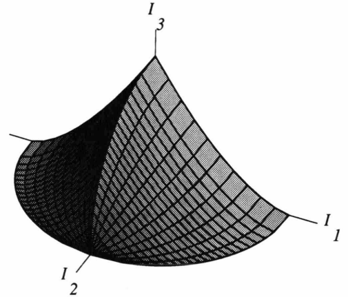
Fig. 2. Energy surface of a cylindrical billiard, h = r = 1 . I_1 is the z -component of the angular momentum, I_2 is the action of motion along the z -direction, and I_3 the action of radial motion.
