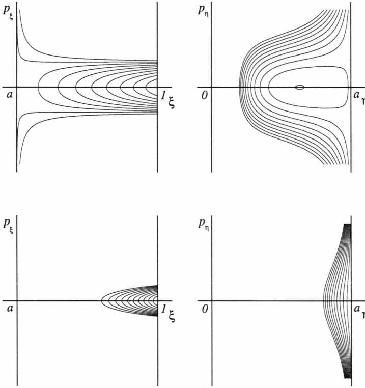
Fig. 9. Phase portraits of billiard motion in an oblate ellipsoid. a = 0.5 , l_\varphi = 0.2 . Left: intersection of invariant tori with the (\xi, p_\xi) -plane; right: intersection of invariant tori with the (\eta, p_\eta) -plane. There are obviously two types of motion. Type I: motion where \xi never gets down to a , i. e., the inner circle is never reached; its stable center is geodesic motion on the ellipsoid, \xi = 1 . Type II: motion where \eta never gets up to a , i. e., the outer ring is never reached; its stable center is motion on the hyperboloid \eta^2 = a|l_\varphi| . The separatrix between the two types consists of orbits that go through the focal circle, \xi = \eta = a .
