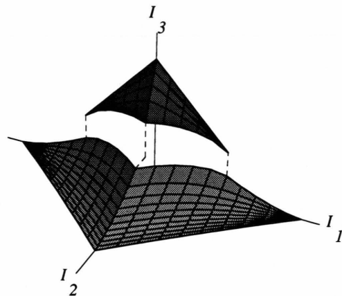
Fig. 11. Energy surface for billiard motion in an oblate ellipsoid. I_1 is the angular momentum component with respect to the symmetry axis; I_2 is the action of \eta -motion; I_3 is the action of \xi -motion. The surface consists of two disconnected sheets, separated along the line of unstable motion in the equatorial plane with angular momentum l_\varphi^2 < a^2 .
