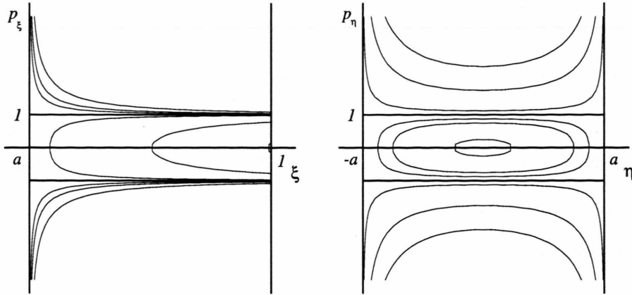
Fig. 3. Phase portraits of the planar elliptic billiard; a = 0.4 , \kappa -values 0.1, 0.3, 0.35, 0.4, 0.45, 0.7, 0.99. Left: intersection of invariant tori with the (\xi, p_\xi) -plane; right: intersection of invariant tori with the (\eta, p_\eta) -plane. The outermost curves of the left picture correspond to the center at right; the outermost curves of the right picture correspond to the point (\xi, p_\xi) \approx (1, 0) . Note that, if this set of pictures is meant to describe motion in the upper half plane, y > 0 , another such set is needed for the lower half plane, y < 0 .
