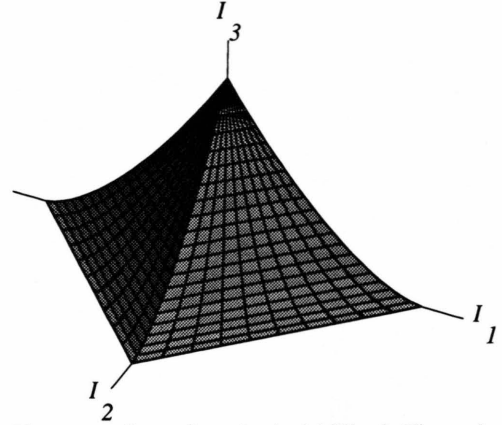
Fig. 1. Energy surface of a spherical billiard. The actions are plotted in units of \sqrt{2E} . I_1 is the z -component of the angular momentum, I_2 the action of the \vartheta -motion, and I_3 the action of radial motion. I_3 depends only on the total angular momentum |I_1| + I_2 . Lines I_3 = \text{const} are drawn for equidistant values of the total angular momentum.
