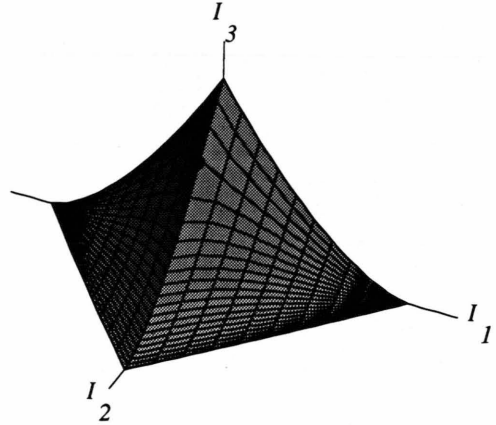
Fig. 8. Energy surface for billiard motion in a prolate ellipsoid. I_1 is the angular momentum component with respect to the symmetry axis; I_2 is the action of \eta -motion; I_3 is the action of \xi -motion. The black dot at (I_1, I_2, I_3) = (0, 2a/\pi, (1 - a)/\pi) marks the singular point which corresponds to motion through the foci.
