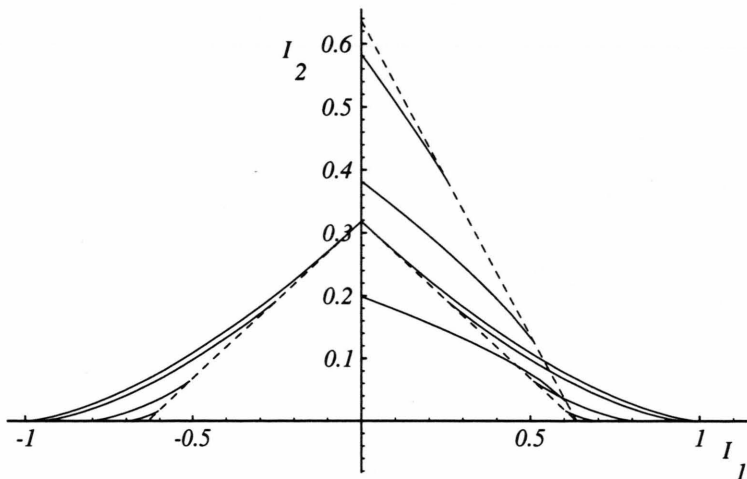
Fig. 4. Energy “surfaces” of elliptical billiards. The action I_1 of (angular) \eta -motion is plotted versus I_2 , the action of (radial) \xi -motion, for different values of a : a = 0, 0.4, 0.8, 0.95 . Note the different scales for I_1 and I_2 . Except for a = 0 , each energy surface consists of three pieces, two with high |I_1| representing rotation of \eta , one with low I_1 and high I_2 , representing motion between the foci. The dotted lines connect the loci of separatrix motion, cf. (28) for the lower branch.
