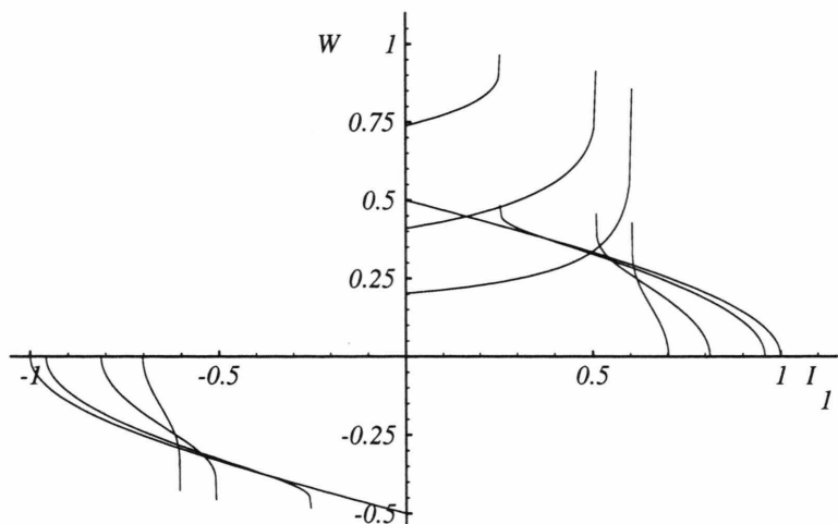
Fig. 5. Winding ratio W_{\eta, \xi} for elliptical billiards, plotted against I_1 . The values of a are the same as in Fig. 4. Separatrices show up with typical logarithmic divergence.
