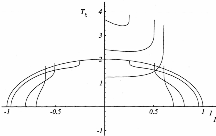
Fig. 6. The period T_\xi of \xi -oscillations as a function of I_1 . The values of a are the same as in Fig. 4.
